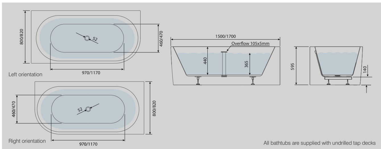
Left hand orientation shown
